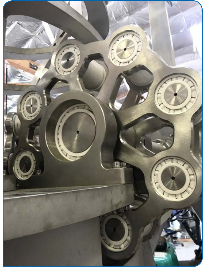
The pinion gear that is part of the energy storage system.
